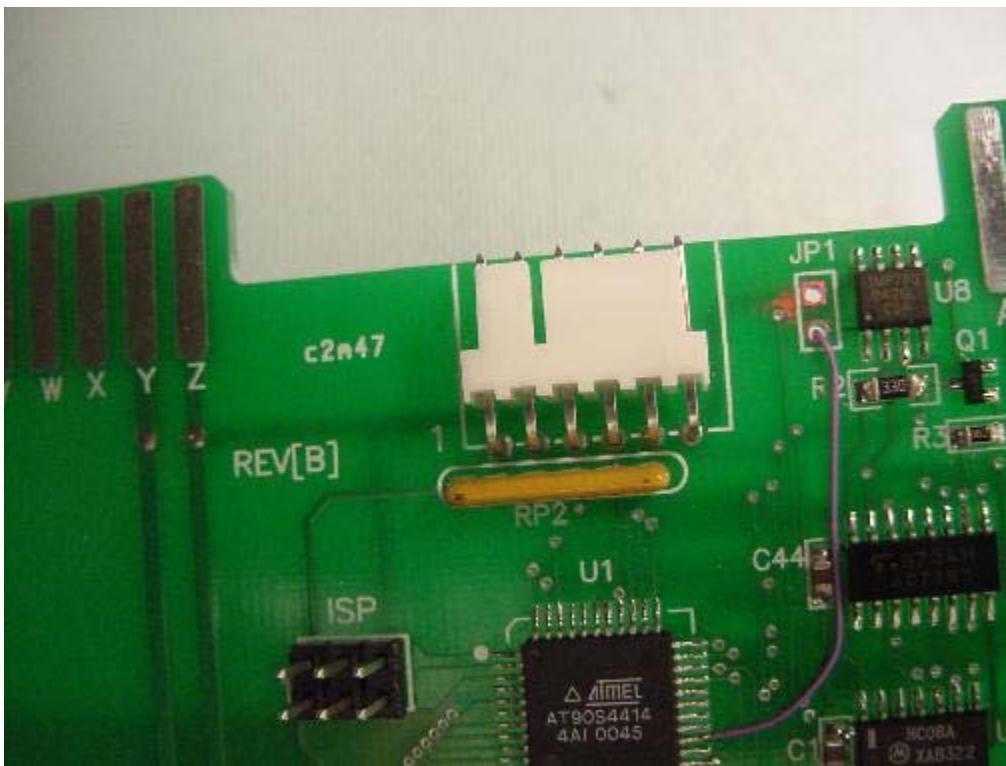
GRAV CONNECTOR – NOTE PIN 1 ON LEFT SIDE
