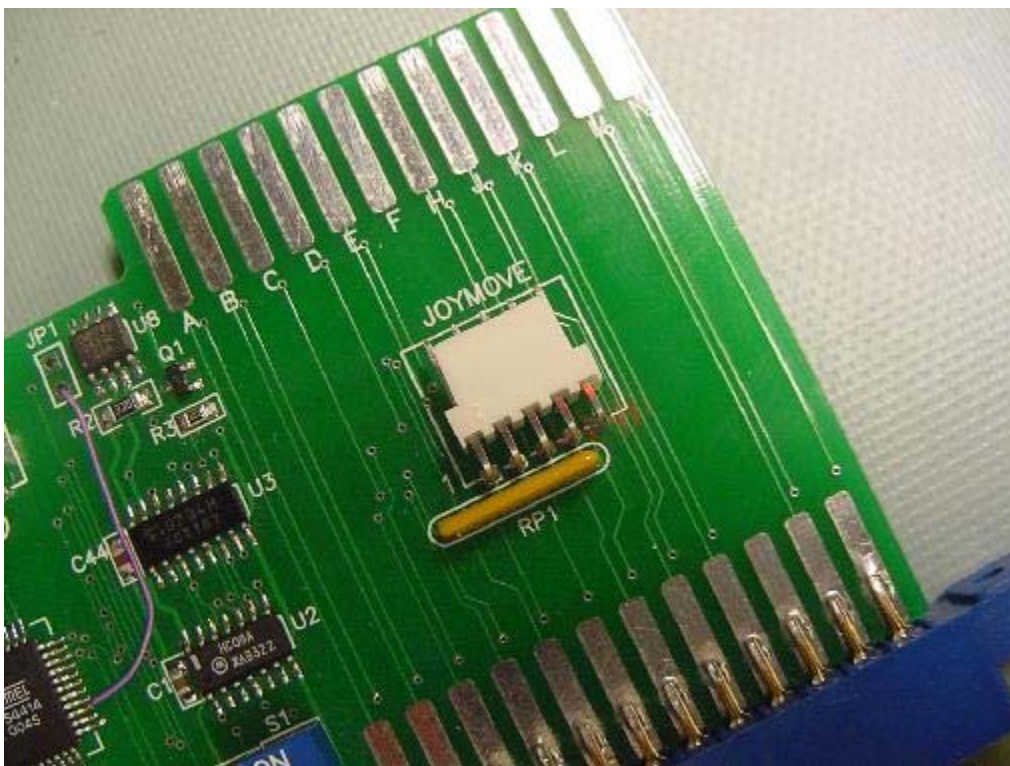
JOYMOVE CONNECTOR = NOTE PIN 1 ON LEFT SIDE
