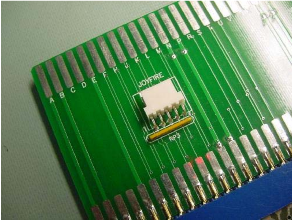
JOYFIRE CONNECTOR – NOTE PIN 1 ON LEFT SIDE
